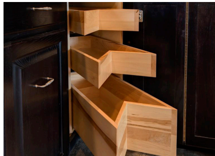
Keypoint Components Lazy Susan Corner Unit with Drawers
