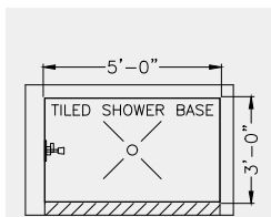
3' x 5' Tiled Shower Base or AKER ICON 6036 AcrylX™ Shower Base (ex. below)
