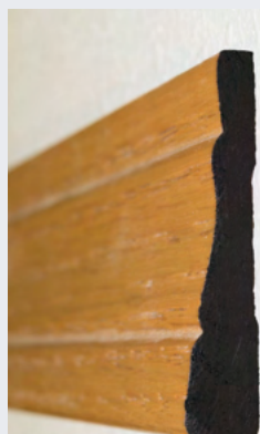
COLONIAL DOOR & WINDOW CASING STANDARD Oak \frac{1}{2} " \times 2\frac{1}{4} " Painted \frac{9}{16} " \times 2\frac{1}{4} " Pine 1\frac{1}{16} " \times 2\frac{1}{4} " Hickory \frac{1}{2} " \times 2\frac{1}{4} "
