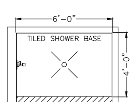
4' x 6' Tiled Shower Base or AKER ICON 7248 AcrylX™ Shower Base
