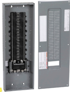
QO160M200PC ELECTRIC SERVICE PANEL (60 Space)
